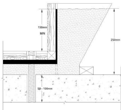
Fig.2 : Typical hopper system
